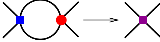
FIG. 3: Schematic of B_K vertex modification due to the insertion of an operator from the staggered action. In the first diagram the (blue) square represents the original B_K vertex and the (red) circle represents the inserted strong four fermion vertex. In the second diagram the (purple) square represents the resulting local vertex in the effective theory.
